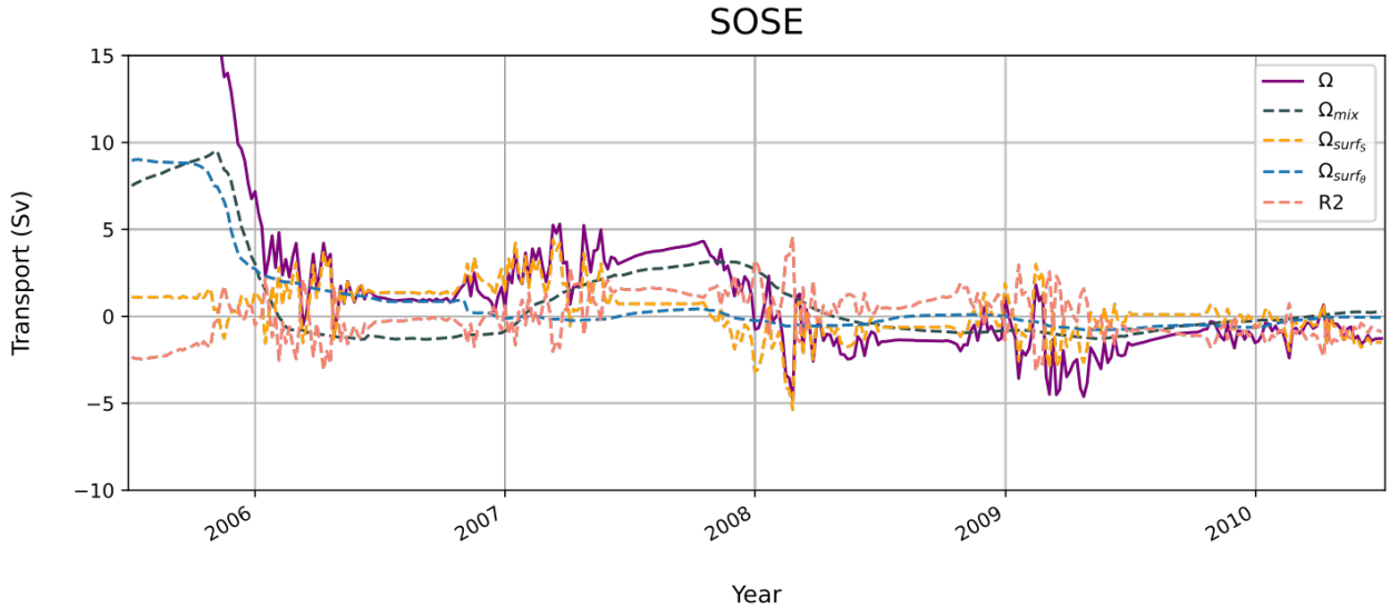
Figure 11. Anomalous transformation term, \Omega (purple solid line), broken down into its sources of transformation: surface salt flux (orange dashed line); surface heat flux (blue dashed line); and mixing (slate grey dashed line). R2 is the pink dashed line.
