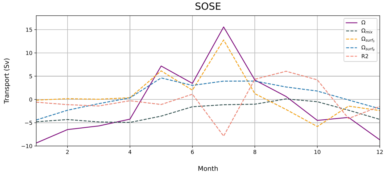
Figure 9. Monthly climatology of Weddell bottom water’s transformation term (purple line), its sources of transformation: surface salt flux (orange dashed line); surface heat flux (blue dashed line); and mixing (slate grey dashed line). Residual due to numerical mixing is the pink dashed line in ECCO (a) and SOSE (b).
