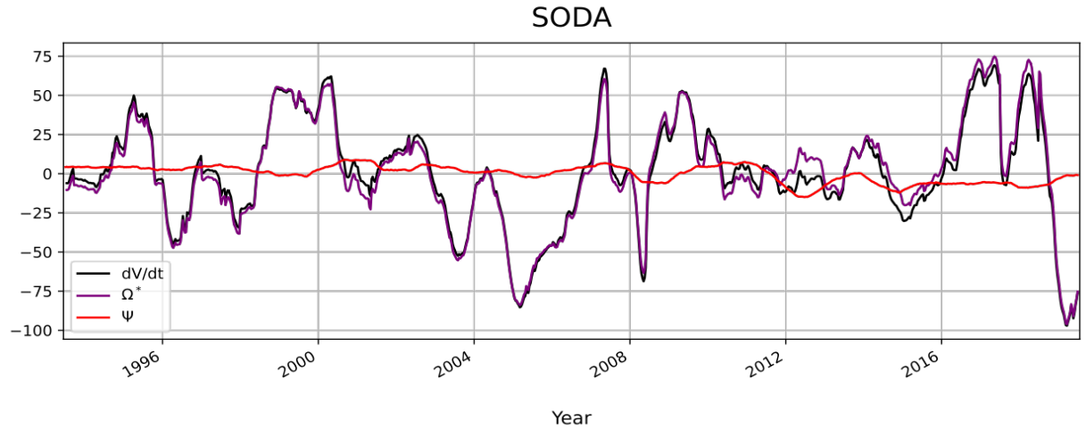
Figure 10. Anomalous main terms of WMT-volume budget in ECCO (a), SOSE (b) and SODA (c). Timeseries was smoothed by an annual rolling mean with the center window set to the middle of the year. Volume change is the black line, transport the red line, transformation is the purple line (includes R2 in ECCO and SOSE, and in SODA also includes R1 and R2), and the discretization residual is explicitly shown as the grey dashed line in ECCO and SOSE.
