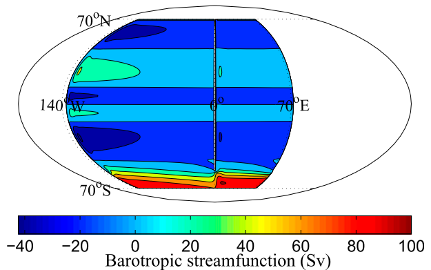
FIG. 4. Barotropic streamfunction and geometry of the domain used in the computations. The domain is 210^\circ periodic and 4000 m deep.
